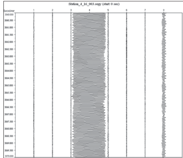
Figure 5 10 s record of the east-west horizontal component of the seismic signal recorded at eight stations on a field delineation project. Dominant ringing at 12 Hz is probably related to compressors operating in the field.
