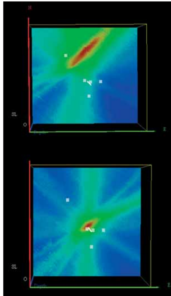
Figure 3 Forward model PSET stacks to correspond with data in Fig. 2. Upper figure anomaly is caused by 3 events at reservoir depth aligned along the length of the red contour. Lower figure anomaly is caused by a single event at perforation point in the well.
