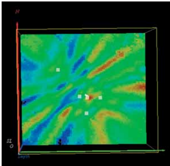
Figure 2 3200 m depth slice through a 50 s PSET stack at onset of flow test. White squares are seismic stations. Test well is at centre station of array. Map is 6 km x 6 km. Hotter colours indicate areas of greater emission energy.
