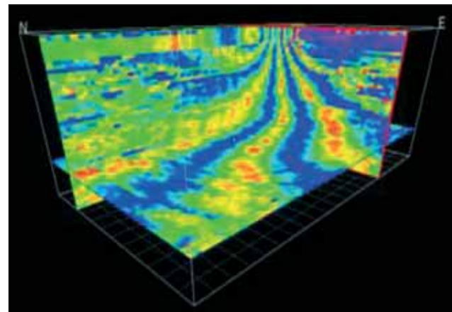
Figure 6 Perspective view of the emission energy stack from the dataset illustrated in Figure 5 showing the effect of the narrow band noise on the stack.
