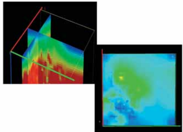
Figure 1 Velocity structure ( V_p ) determined from passive seismic. Depth slice is 60 x 60 km at 2 km depth. Base of green in depth cube is at about 6 km. Velocities range from 1800 m/s (blue) to 6500 m/s (red)
